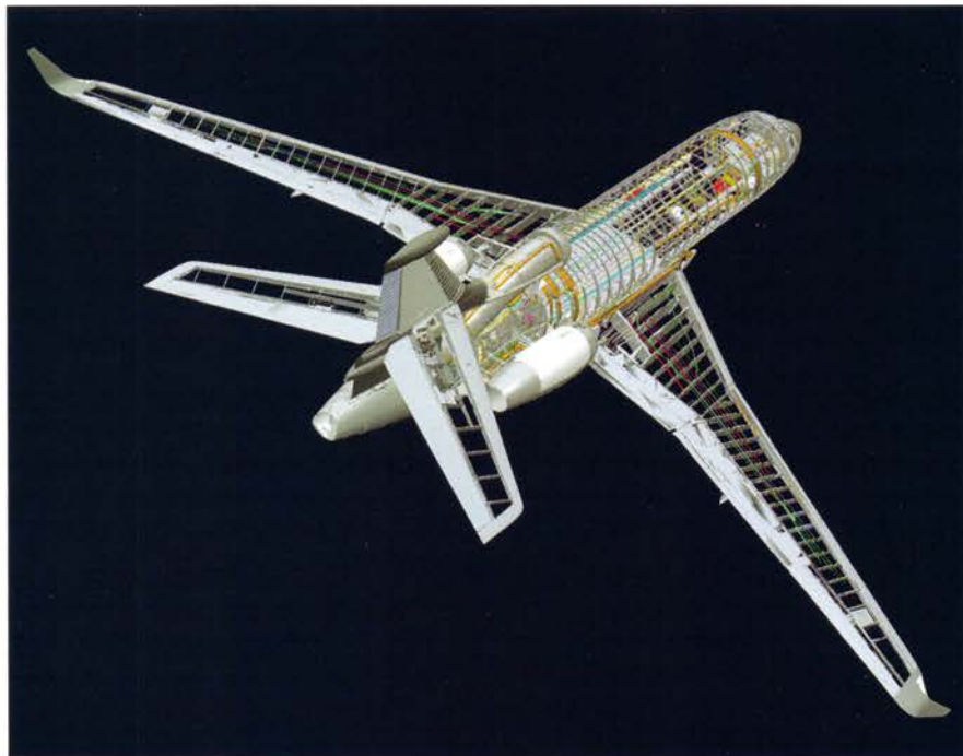
The new Falcon's fuselage has a heavier duty substructure, enabling cabin pressurization to be increased even though it has larger cabin windows than the Falcon 900.
